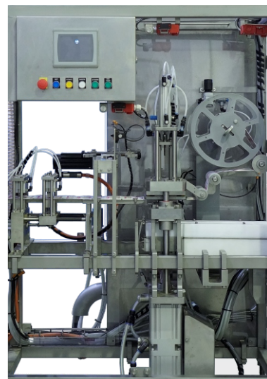
. Automatizada con PLC y panel HMI . Automated with PLC and HMI
